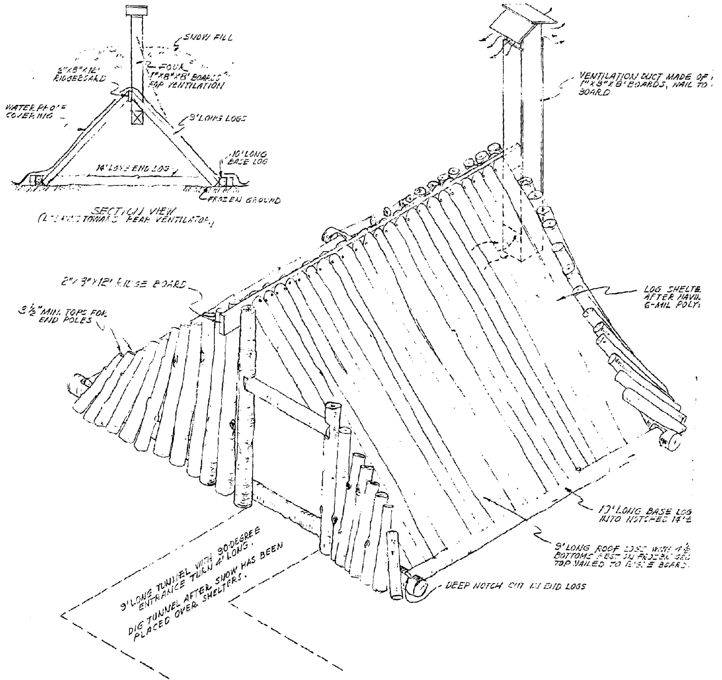
Fig. A-4.2. Two-Family A-Frame Pole Shelter, Frozen Ground Version.
